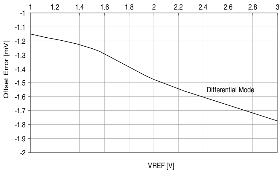
Figure 36-50. Offset Error vs. External V_{REF}
