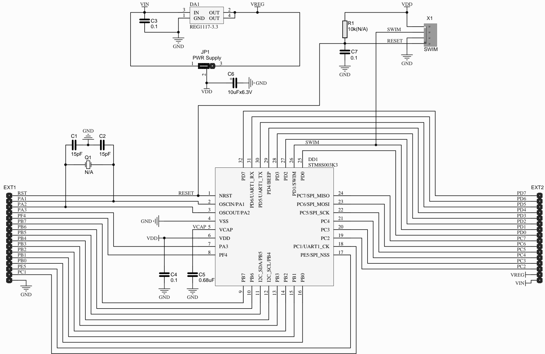
STM8S-DIP-LQFP32
