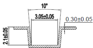
Figure 5: Carrier tape dimensions
