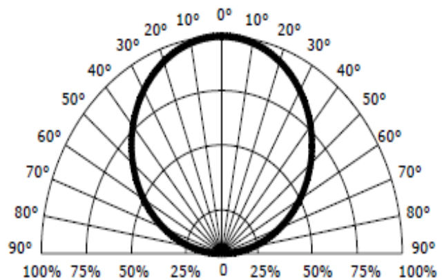
Fig. 6 Relative Luminous Flux vs Radiation Angle
