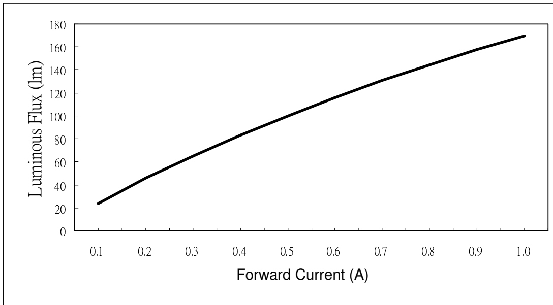
< Figure 7. Forward current & relative luminous at T_a=25^\circ\text{C} for 1W PLCC >
