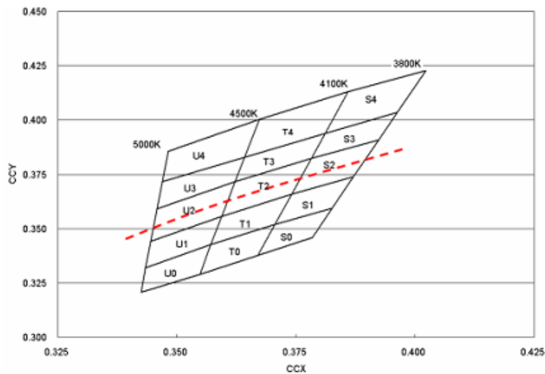
< Figure 4 PLCC Chromaticity diagram >
