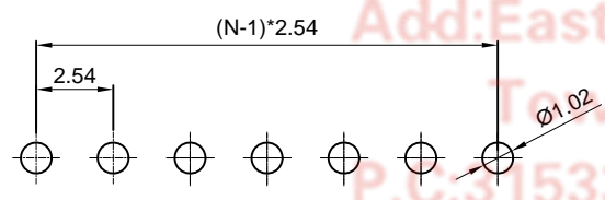
Recommend PCB Layout (Tolerance=±0.05)
