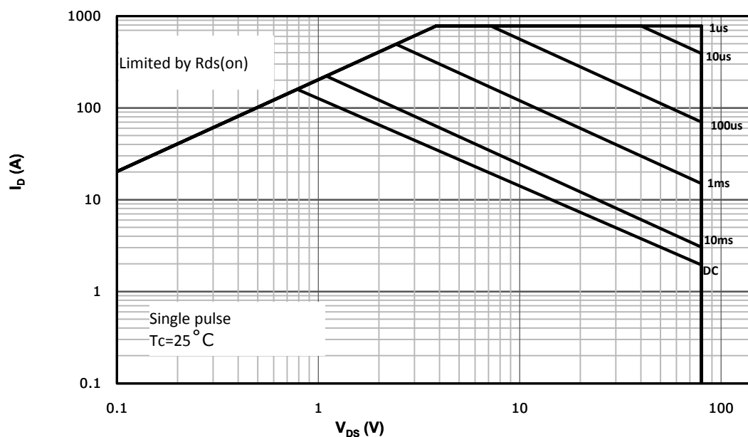
Fig 13: Safe Operating Area
