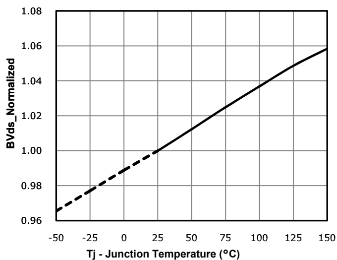
Fig 11: BVds vs. Temperature
