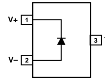
Figure 1. 3-Lead SC70 (KS) and 3-Lead SOT-23 (RT)
