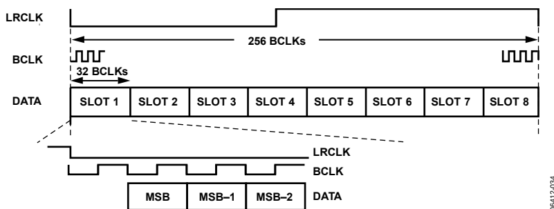
Figure 35. TDM Mode
