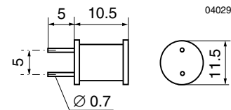
Fig. 9 Dimensions for inductor L
