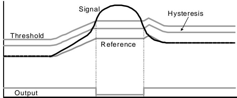
Figure 2.5 Drift Compensation
