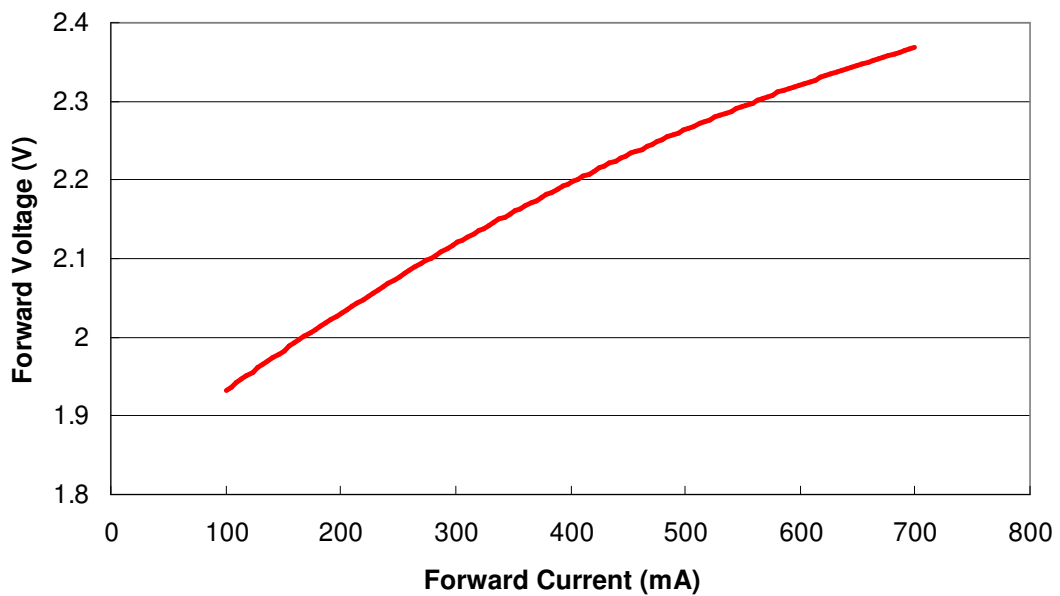
Figure 10: Forward voltage vs. forward current for Red and Amber.
