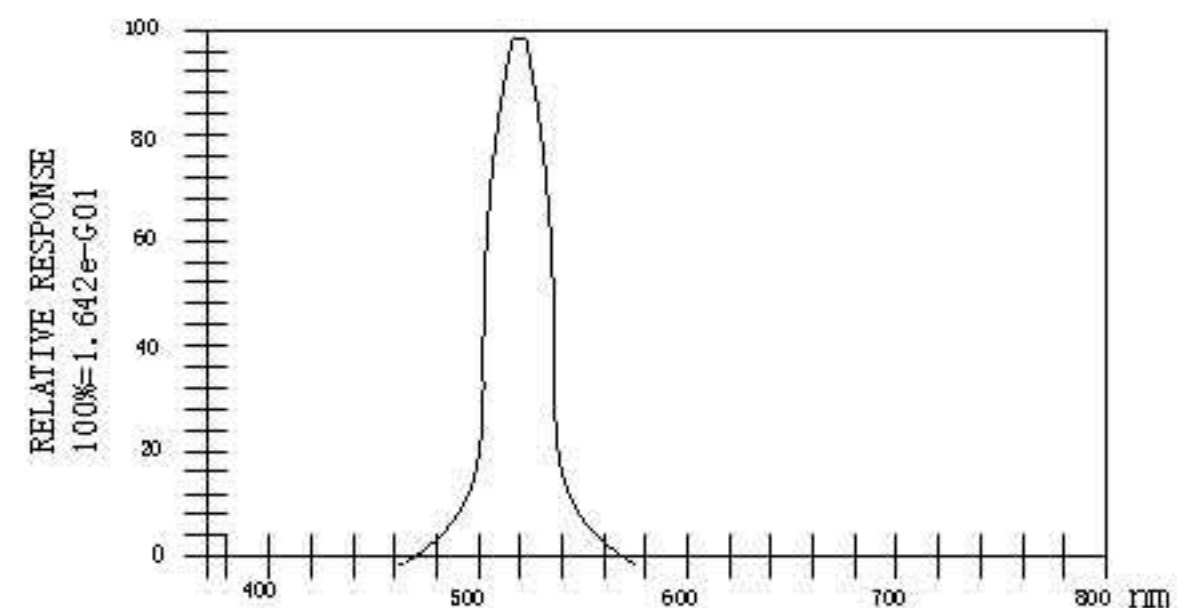
Luminous Spectrum (Ta=25°C) SPECTRAL RADIANCE
