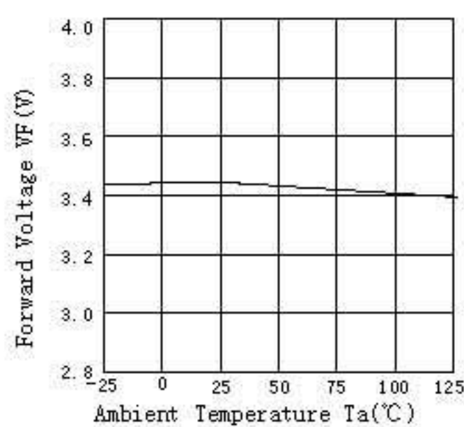
Forward Voltage vs. Ambient Temperature
