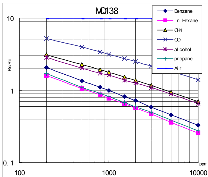
Fig.2 sensitivity characteristics of the MQ-138
